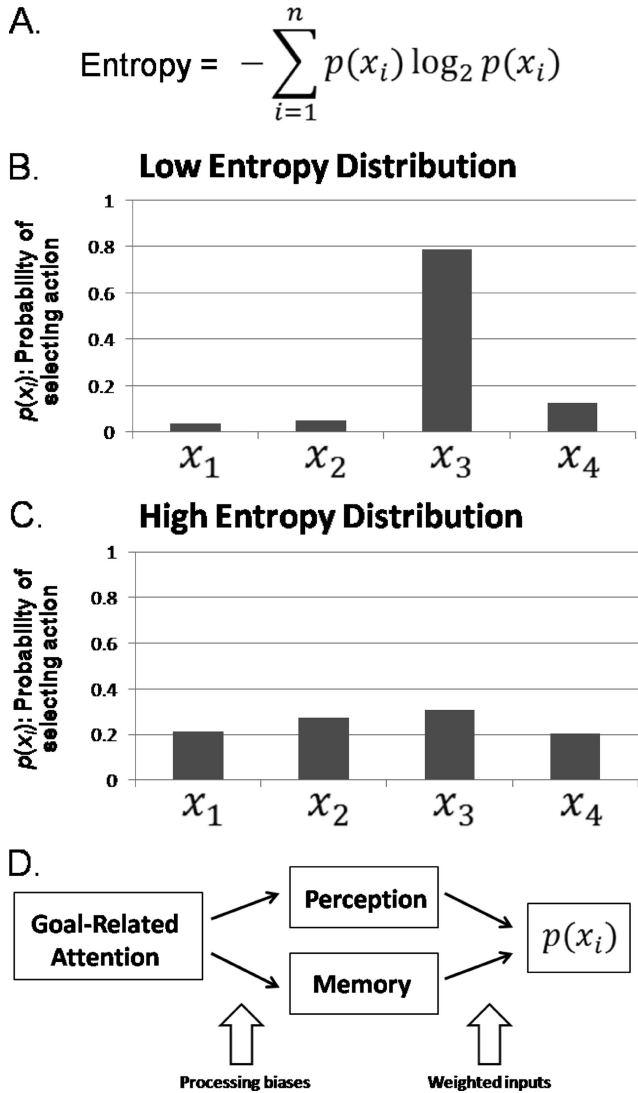
Figure 1. A: Shannon’s formula for information entropy. Entropy increases as the number of possible outcomes increases and the probability of any particular outcome, p(x_i) , decreases. B: Low psychological entropy occurs during situations in which there is a high probability of employing a particular action or perceptual frame, x_i . C: High psychological entropy occurs during situations in which there are multiple competing frames and behavioral options (e.g., x_1, x_2, x_3 ), none of which is clearly more strongly activated than the others. D: The probability of any given action or perceptual frame being employed, p(x_i) , is a function of the weighted neural input for its deployment, as influenced by the combination of sensory input, strength of memory representations, and goal-related attentional processes.
